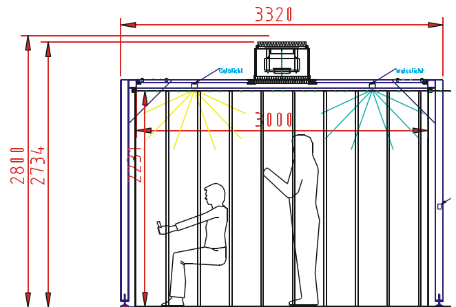
Fig. 2 cross section clean room cell
